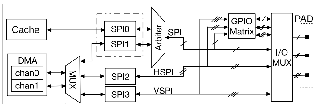
Figure 20.1-1. SPI Architecture
