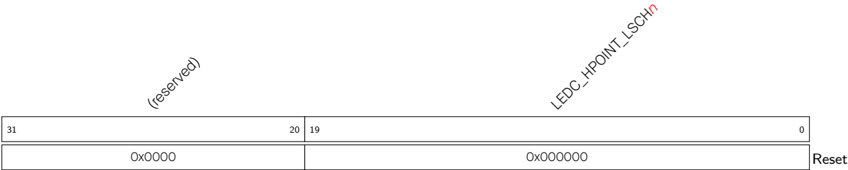
Register 28.7. LEDC_LSCH n _HPOINT_REG ( n : 0-7) (0xA4+0x14* n )
