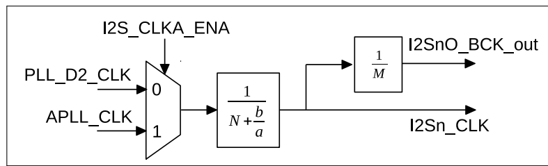
Figure 22.3-1. I2S Clock
