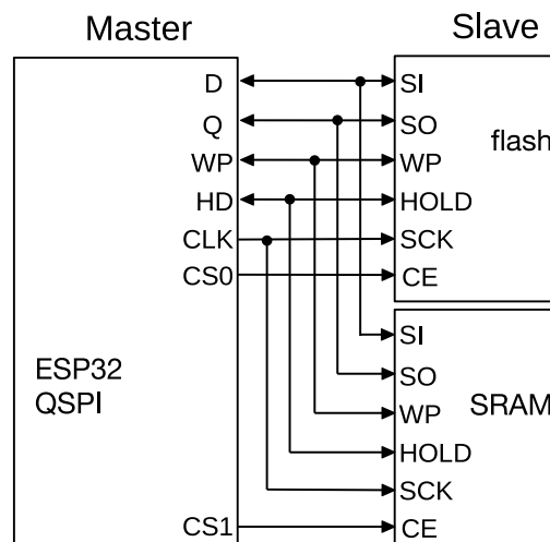
Figure 20.5-1. Parallel QSPI
