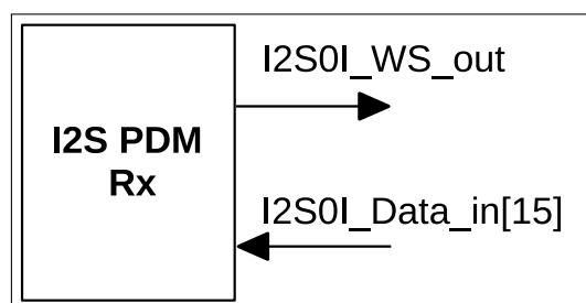
Figure 22.4-9. PDM Receives Signal
