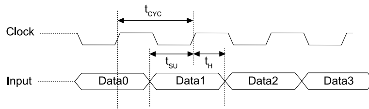
Figure 24.6-5. RMII Timing - Receiving Data
