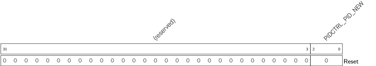
Register 13.13. PIDCTRL_PID_NEW_REG (0x048)
