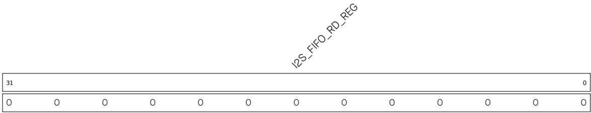
Register 22.2. I2S_FIFO_RD_REG (0x0004)
