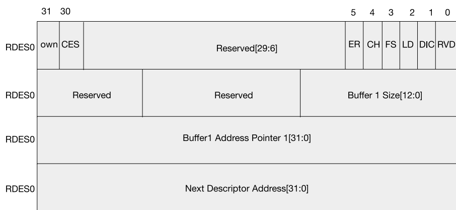
Figure 27.8-1. The Structure of a Linked List
