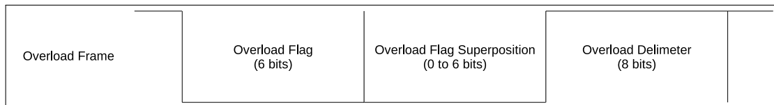
Figure 25.3-3. The Bit Fields of an Overload Frame
